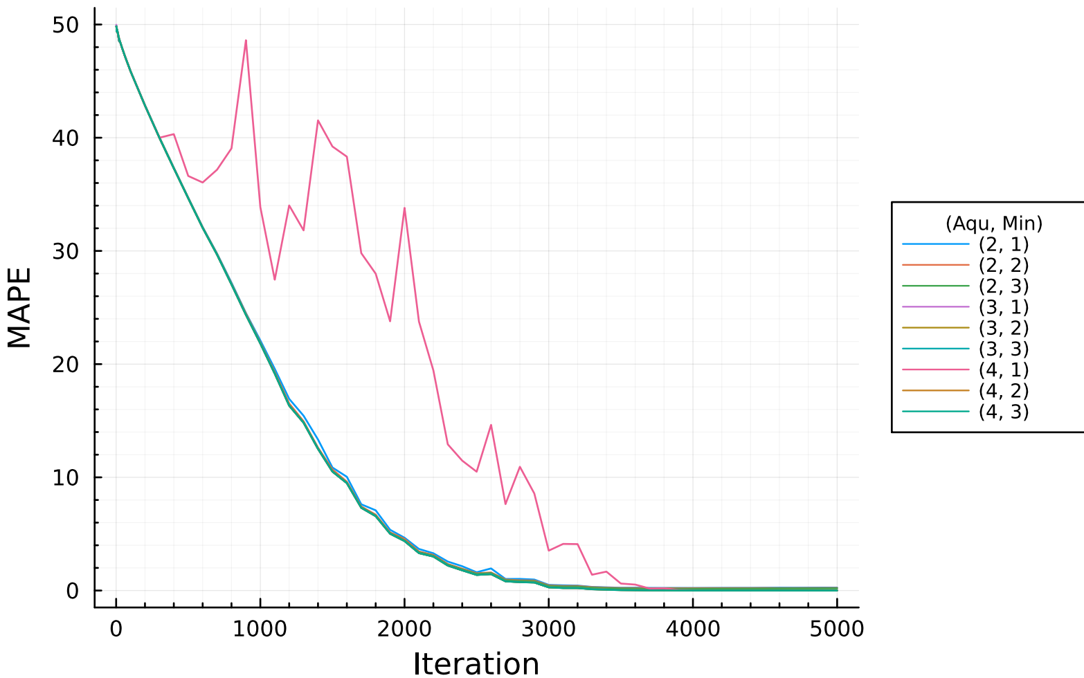
MAPE Ba vs. Iteration
