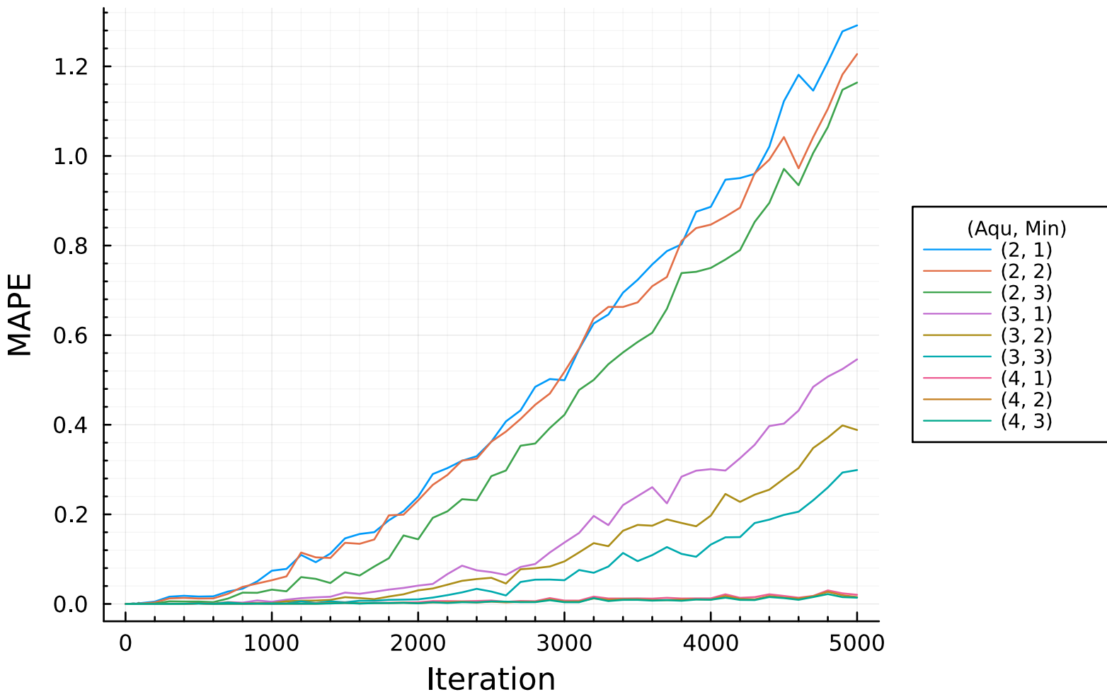
MAPE Barite vs. Iteration
