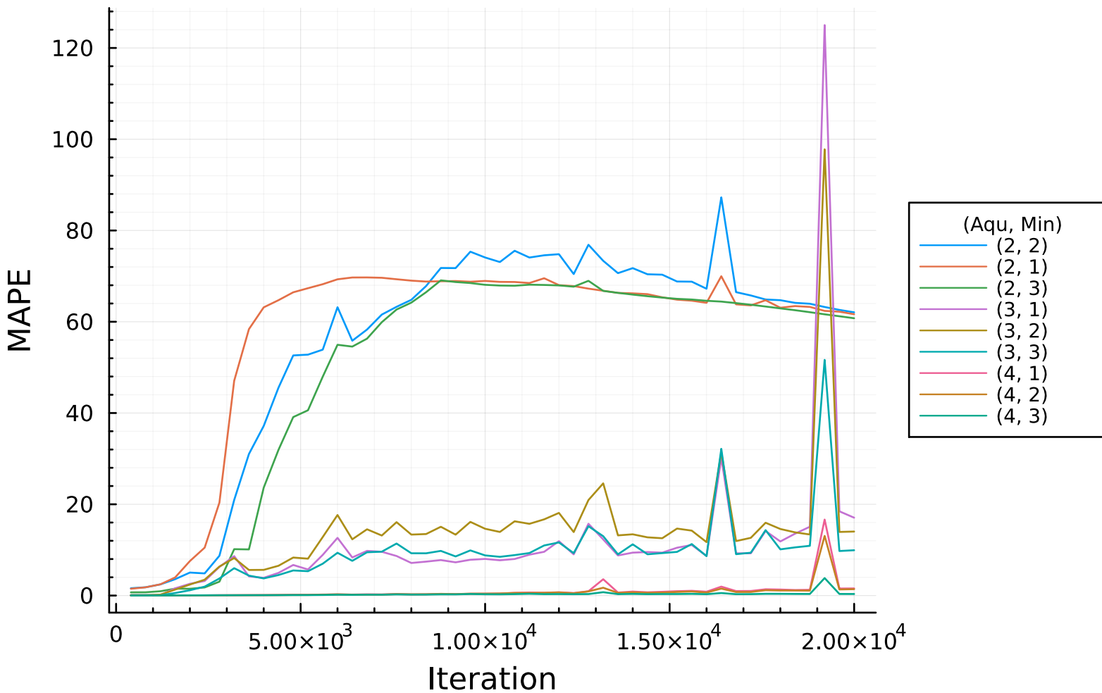
MAPE Calcite vs. Iteration
