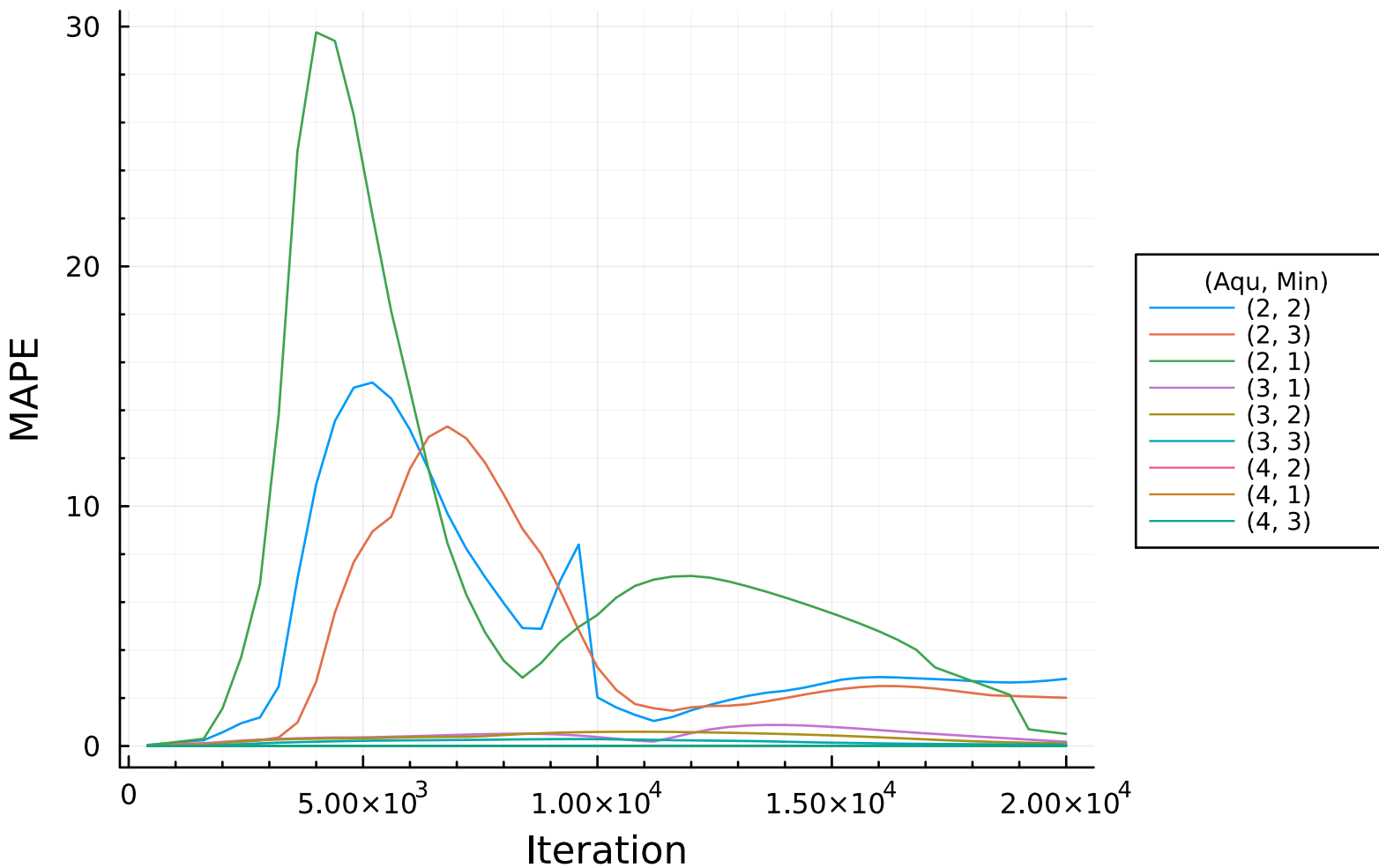
MAPE Mg vs. Iteration
